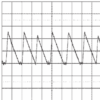
Figure 36. Transition Mode Operation V_{\text{IN}} = 24 \text{ V} , V_O = 3.3 \text{ V} , I_O = 0.29 \text{ A}
