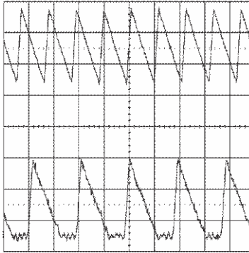
Figure 35. CCM and DCM Operating Modes V_{\text{IN}} = 12 \text{ V} , V_O = 3.3 \text{ V} , I_O = 1 \text{ A} / 0.25 \text{ A}
