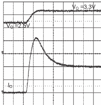
Figure 33. Prebiased Start-Up
