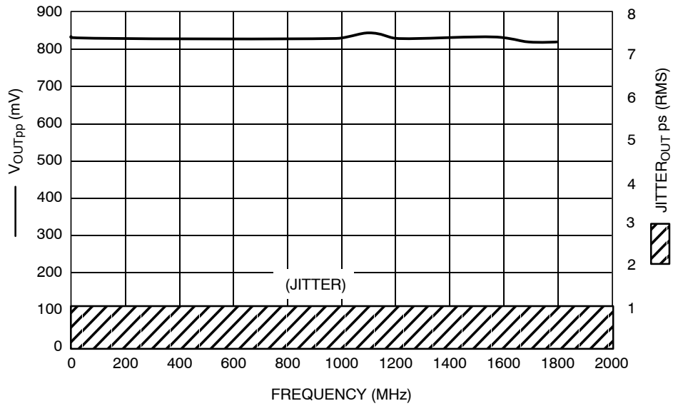
Figure 6. \div 5 , F_{\max}/\text{Jitter}
