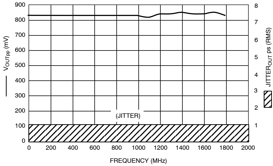
Figure 5. \div 2 , F_{\max}/\text{Jitter}
