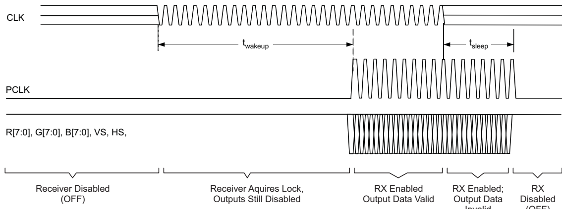
Figure 15. Standby Detection
