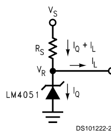
FIGURE 1. Shunt Regulator
