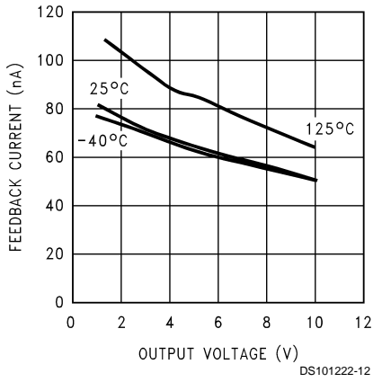
Feedback Current vs Output Voltage and Temperature
