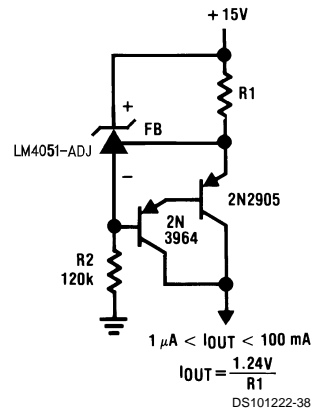
FIGURE 11. Current Source
