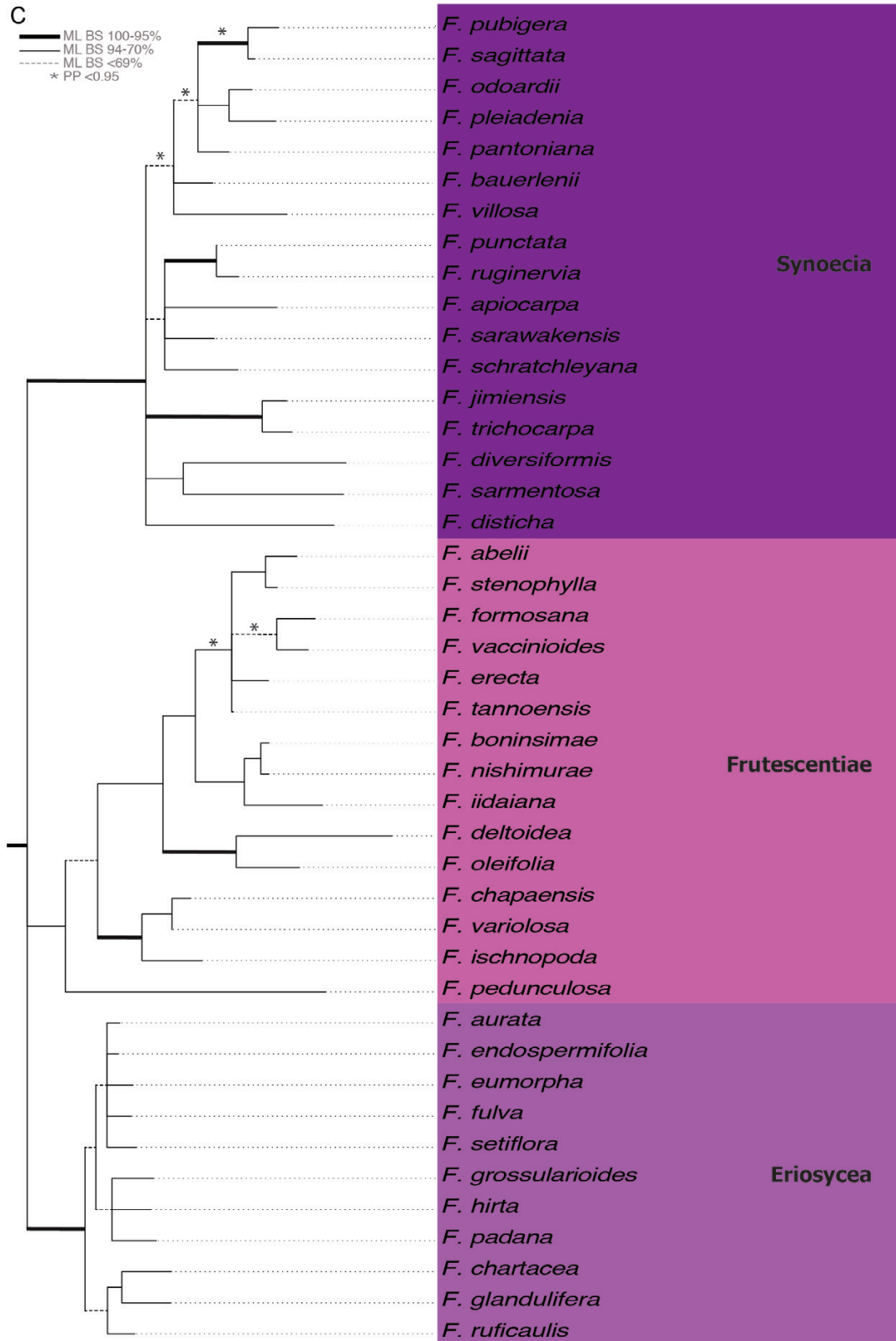
Figure 3A–F. Maximum likelihood tree of the combined analysis of six gene regions for 307 Ficus spp. ML bootstrap support indicated as follows: thickened branches = 95–100%, thin branches = 70–94% and dashed branches = < 69%;
