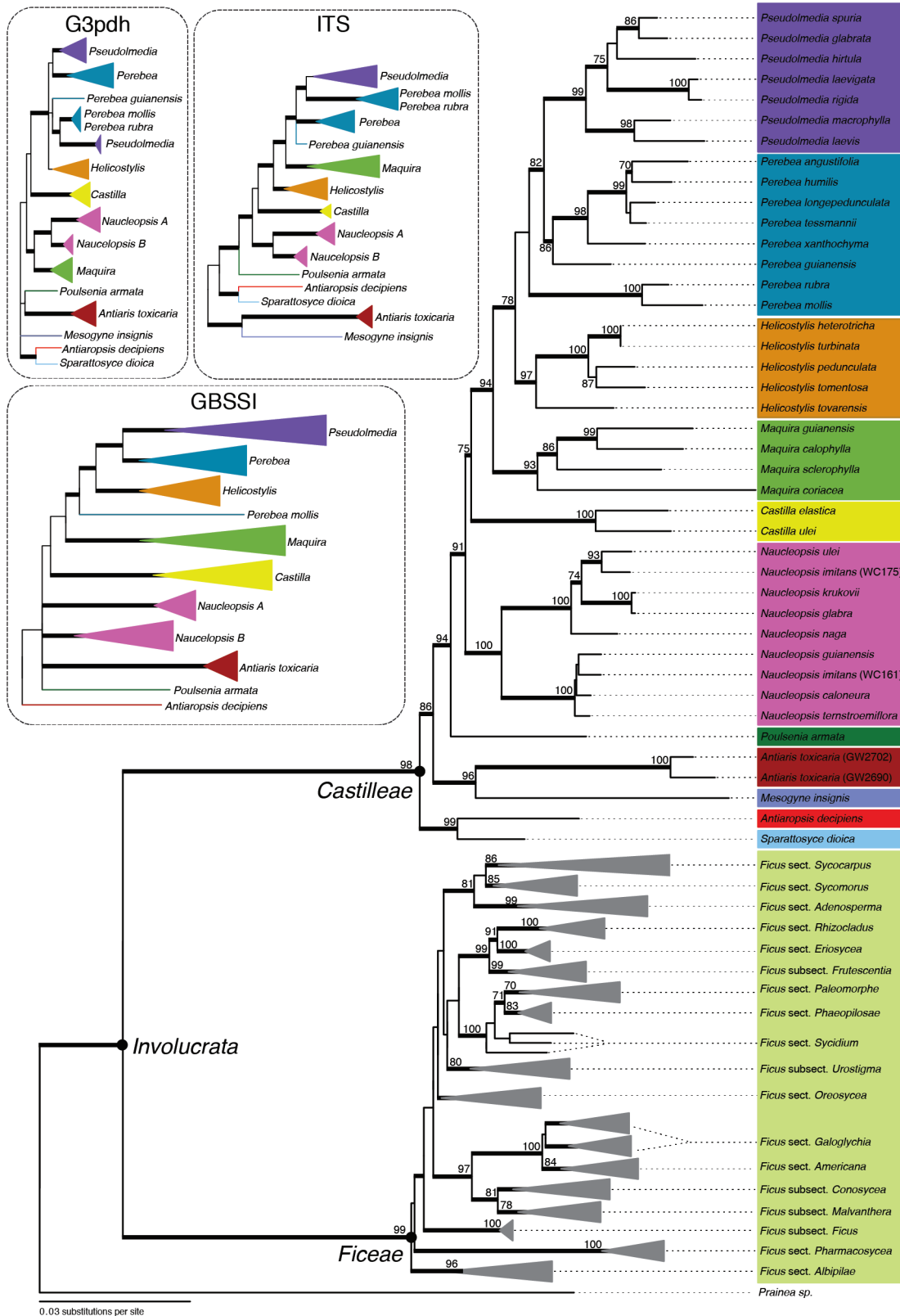
Figure 1. Phylogenetic trees from individual (upper left panel) and combined (main tree) maximum likelihood analyses of Involucrata using ITS, G3pdh and GBSSI . Thickened branches represent posterior probabilities greater than 0.95, and maximum likelihood bootstrap values are indicated above the branches (main tree only). Genera in Involucrata are
